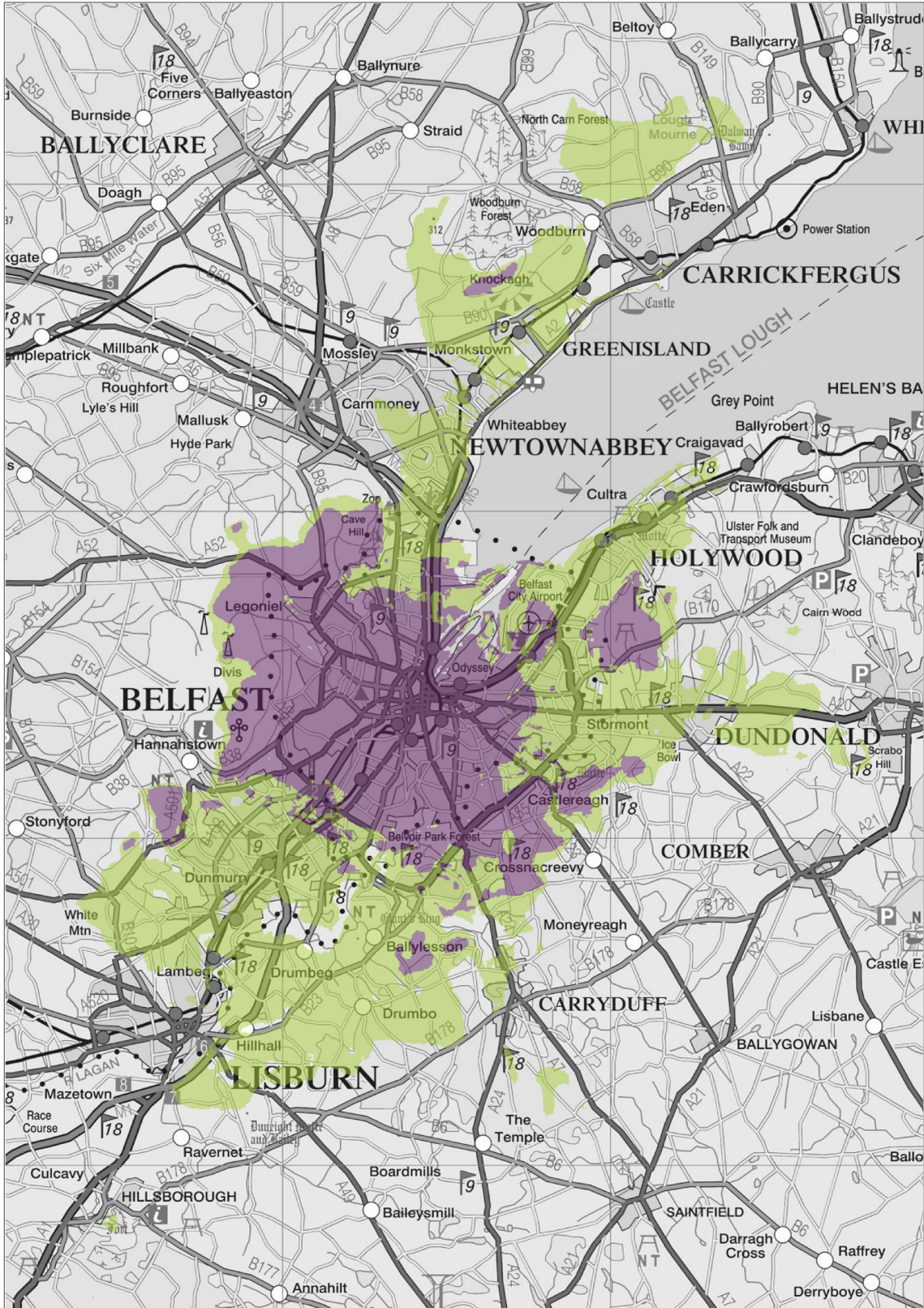
Predicted Coverage ( 64 dBµV/m, 54 dBµV/m) for Belfast 89FM on 89.3 MHz at 100W HP & 100W VP
